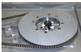
A precision ring bearing and Orion's DuraGlide cams provide reliable support for loads weighing up to 5,000 pounds.
